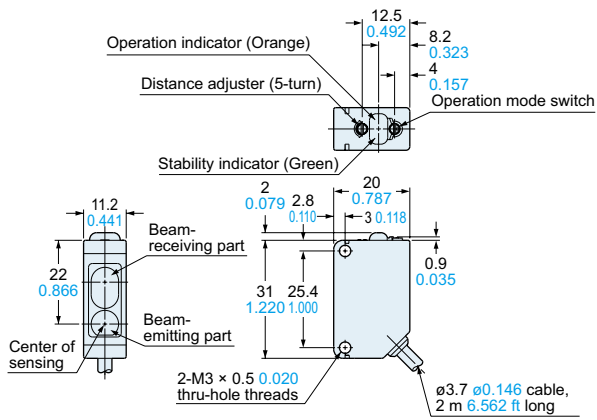
CX-44□ Sensor
