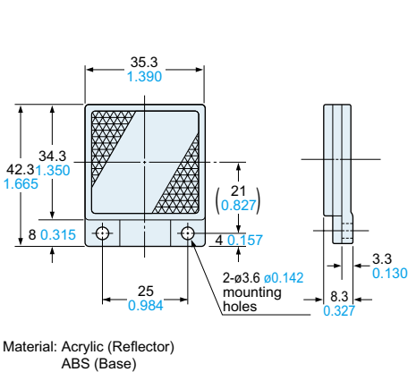
RF-220 Reflector (Optional)
