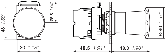
MPET4 Dimensions (mm, inches)
